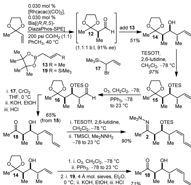
Scheme 2. An efficient synthesis of hydrazone 2 in just 5 steps. TESOTf = triethylsilyl triflate, TMSCl = trimethylsilyl chloride.
